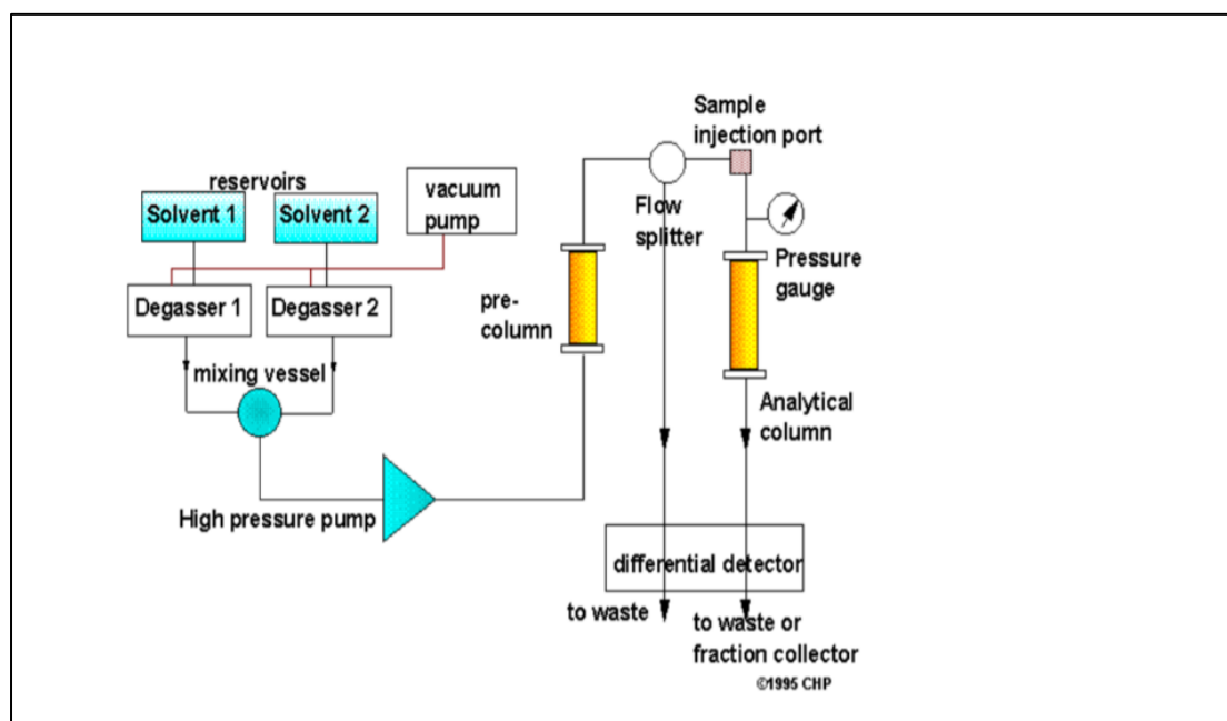
Figure 1: Schematic Diagram of High-Performance Liquid Chromatography
