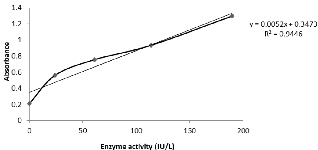
Standard curve for SGOT
