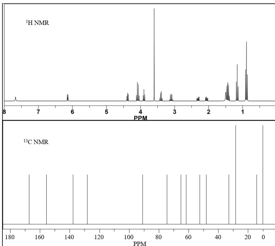
Fig. 3: Estimation of OP by NMR.
