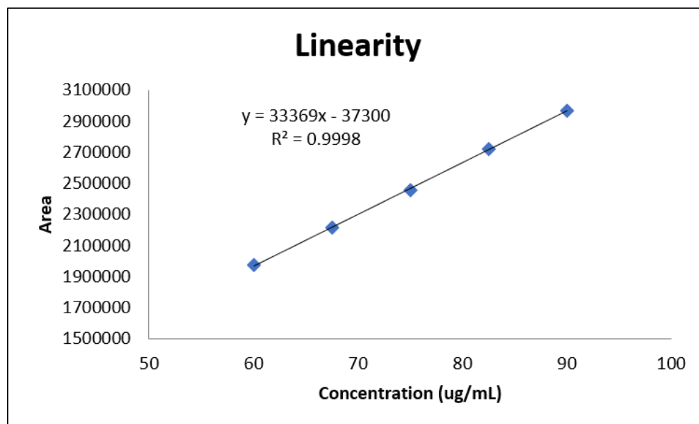
Fig. 8 Calibration curve of linearity study.
